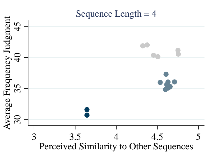
Figure A4. Similarity to average sequence predicts estimated frequency. Each dot corresponds to a coin-flip sequence of length four. The x-axis shows the average judged similarity between that sequence and other sequences of the same length. The y-axis shows the average belief about the likelihood of that sequence (per 500 four-flip sequences).
