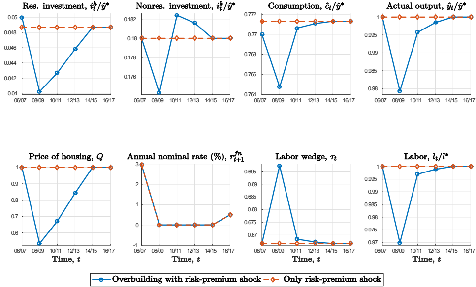
Figure 8: Calibration with overbuilding and risk-premium shocks.
