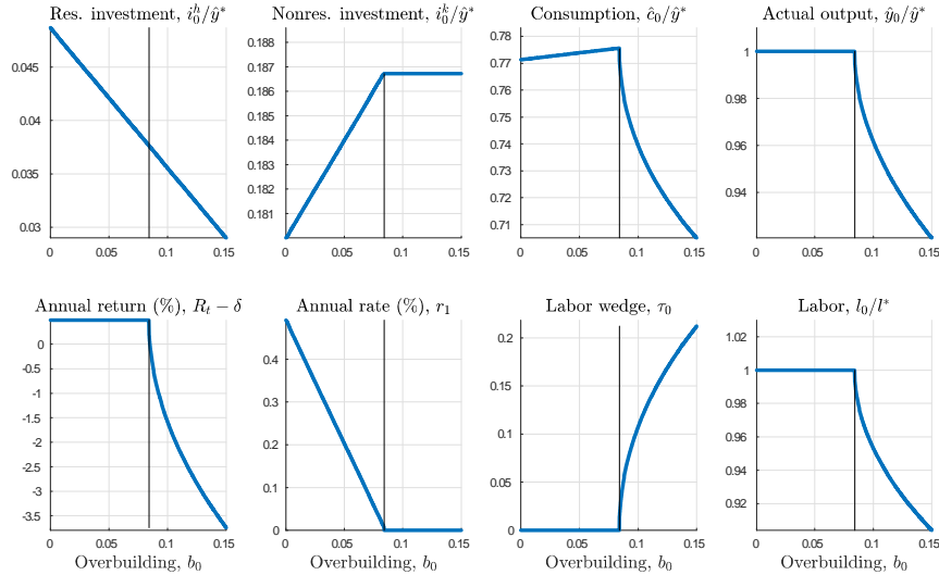
Figure 3: Date 0 equilibrium variables as a function of the initial overbuilding b_0 (measured as a fraction of the steady-state residential capital stock, h^* ).
